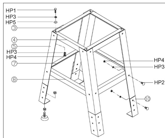
Figure 10: stand assembly (optional accessory)
