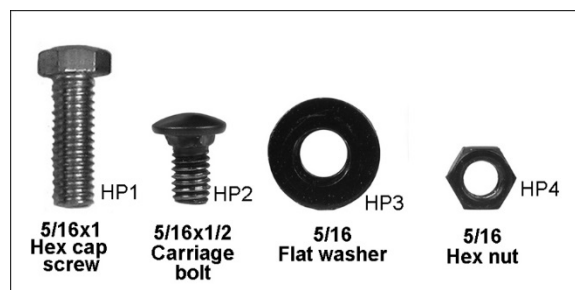
Figure 5: hardware package JWSS22B-SHP
