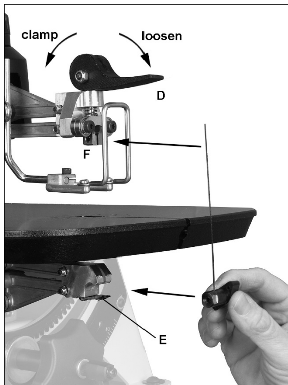
Figure 15: installing blade into guides
