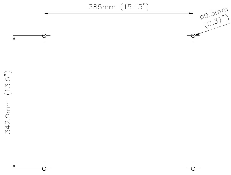
Figure 2: scroll saw mounting hole pattern
