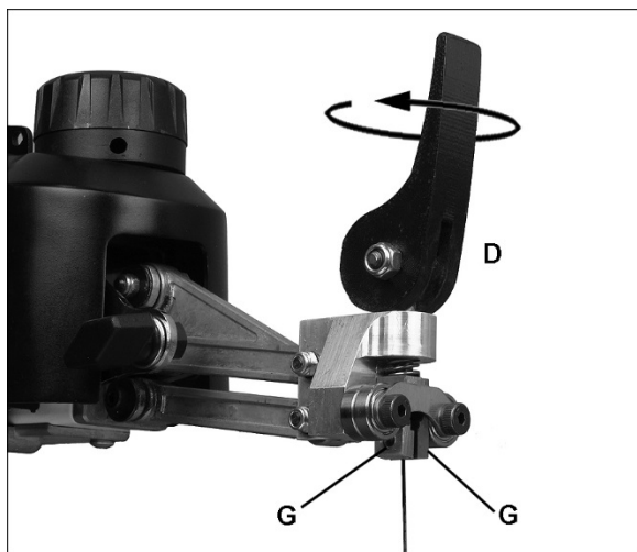
Figure 17: tension adjustment
