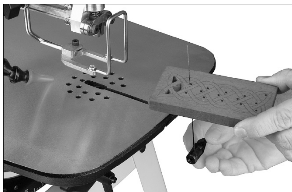
Figure 16: installing blade with workpiece
