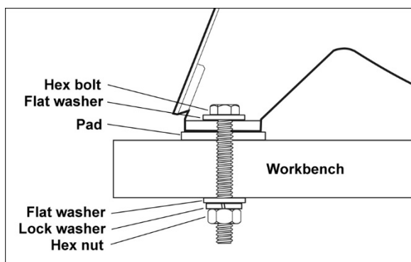
Figure 9: bench mounting (fasteners not included)
