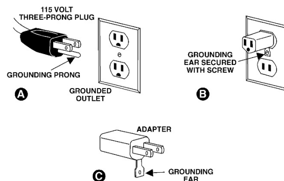
Figure 12: plug configuration
