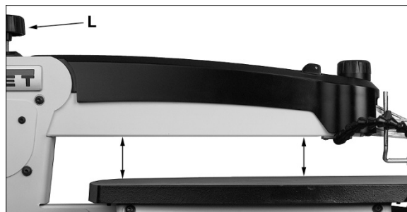
Figure 22: arm/table parallelism
