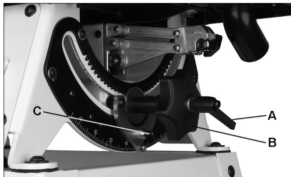
Figure 13: arm tilt adjustment
