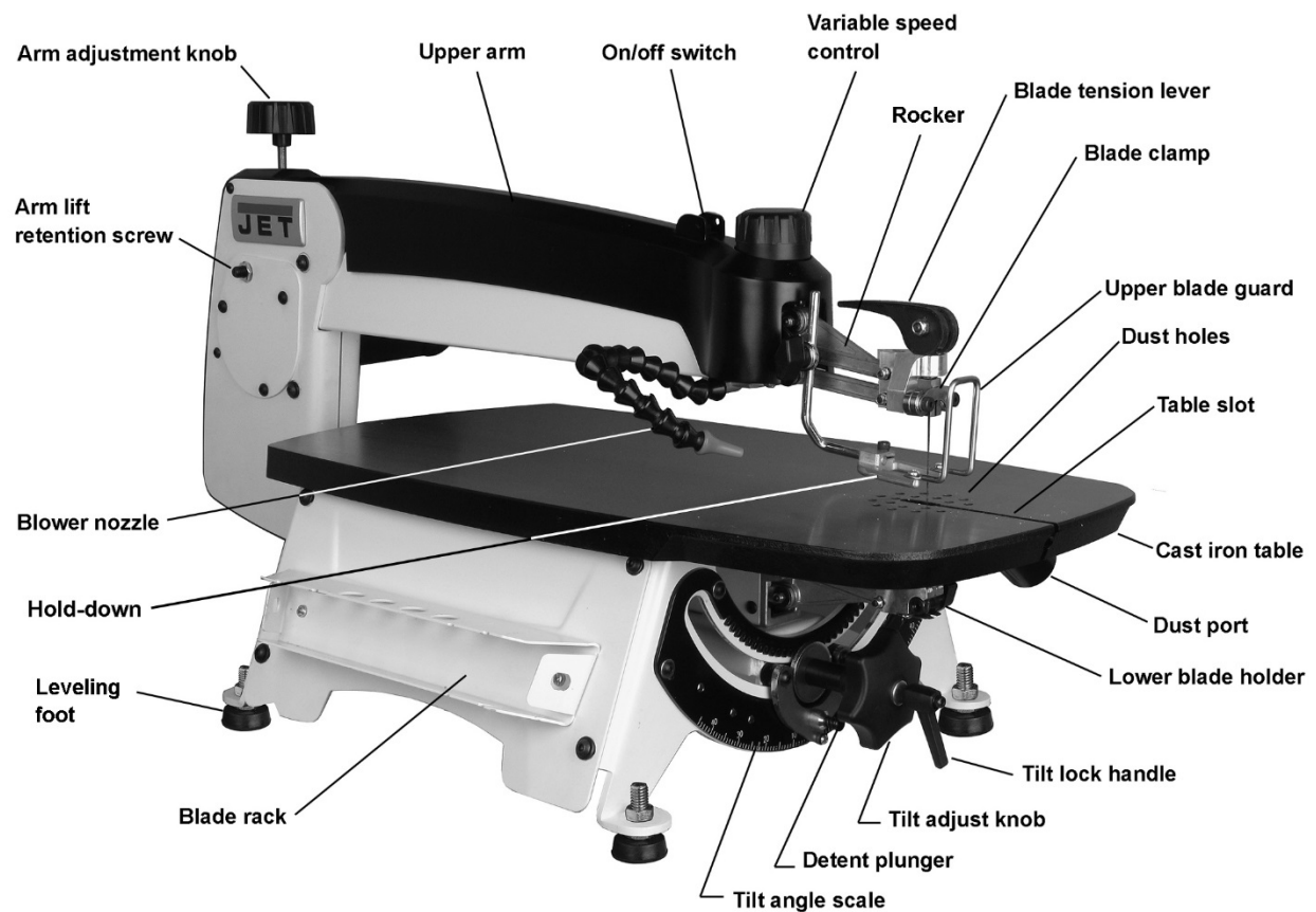
Figure 3: JWSS-22B features
