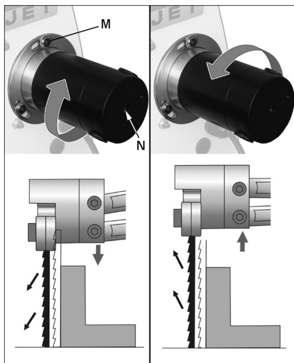
Figure 23: blade oscillation
