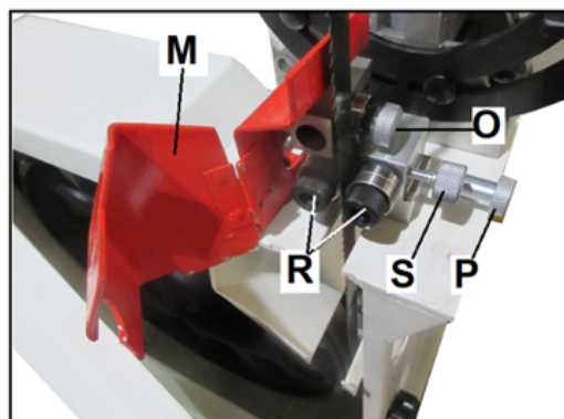
Figure 5-12: lower blade guides
